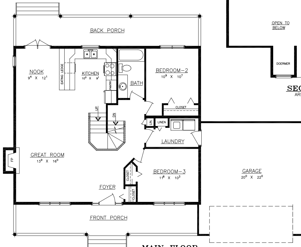
MAIN FLOOR AREA = 1807 S.F.
